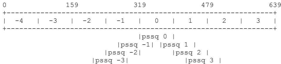
Figure 7.4. Enhancement for 30 ms frame size
