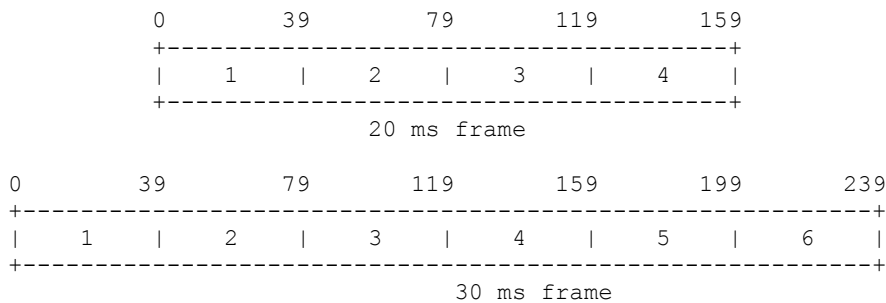
Figure 6.2. One input block to the encoder for 20 ms (with four sub-frames) and 30 ms (with six sub-frames)
