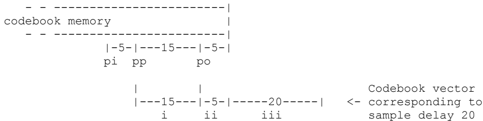
Figure 6.11. Generation of the first augmented codebook
